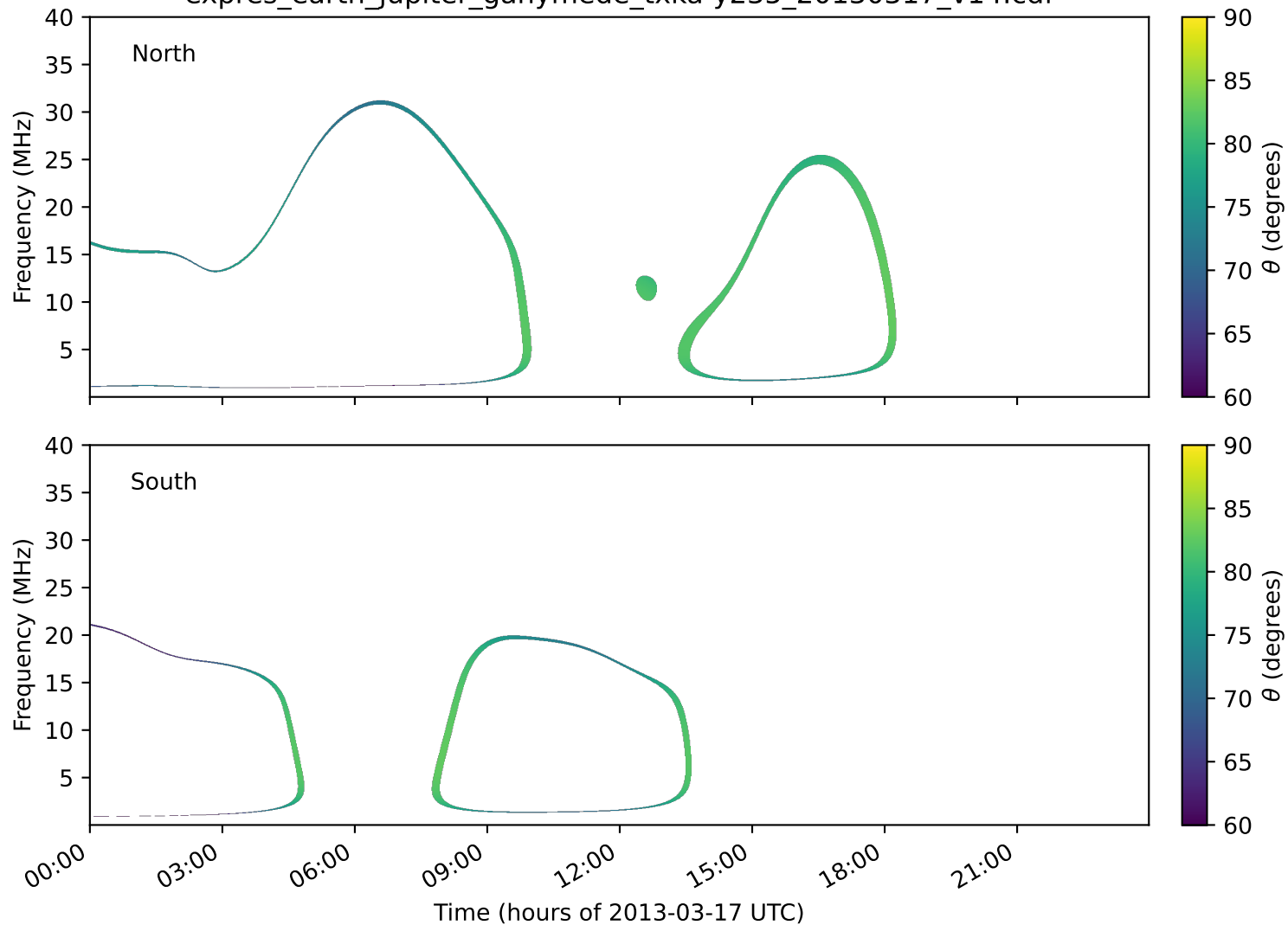
expres_earth_jupiter_ganymede_txka-y235_20130317_v14.cdf
