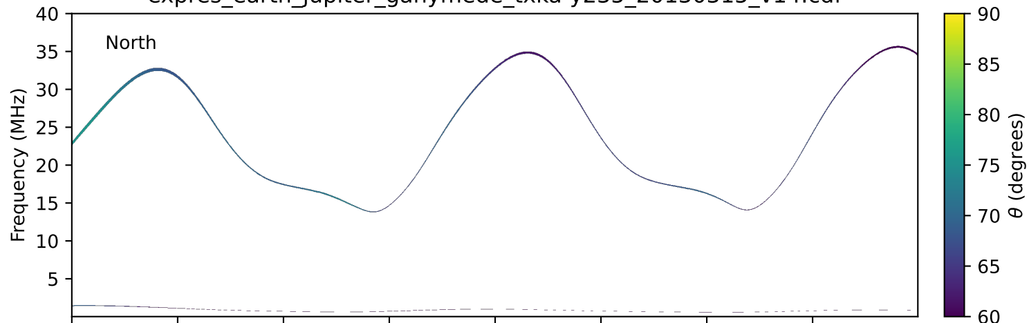
expres_earth_jupiter_ganymede_txka-y235_20130315_v14.cdf
