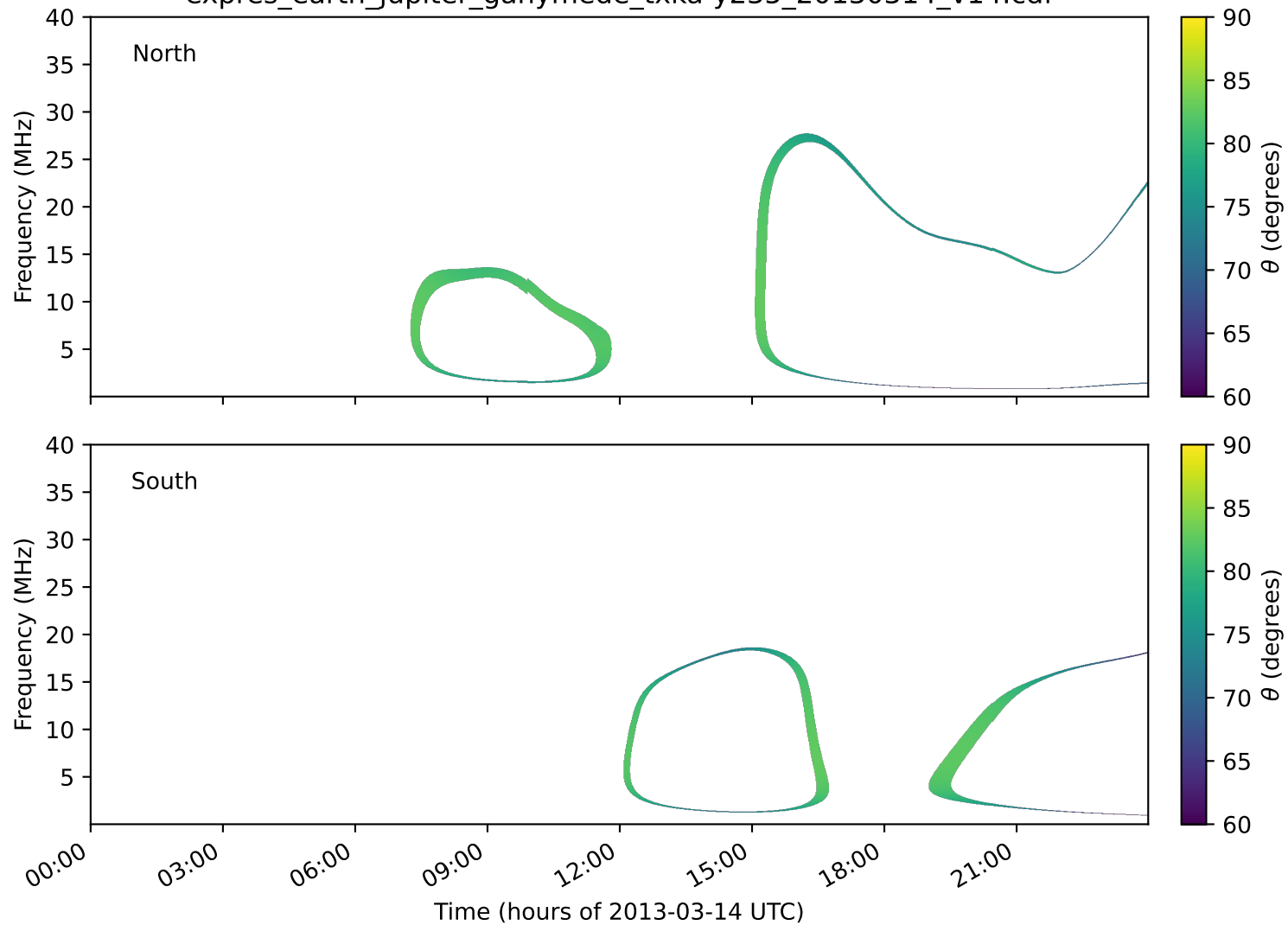
expres_earth_jupiter_ganymede_txka-y235_20130314_v14.cdf
