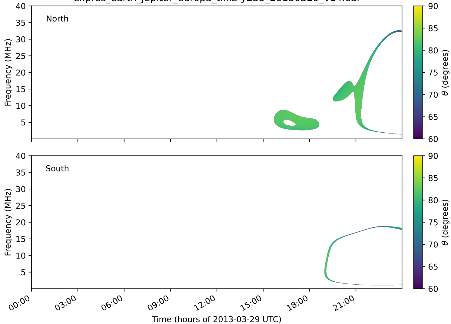
expres_earth_jupiter_europa_txka-y235_20130329_v14.cdf
