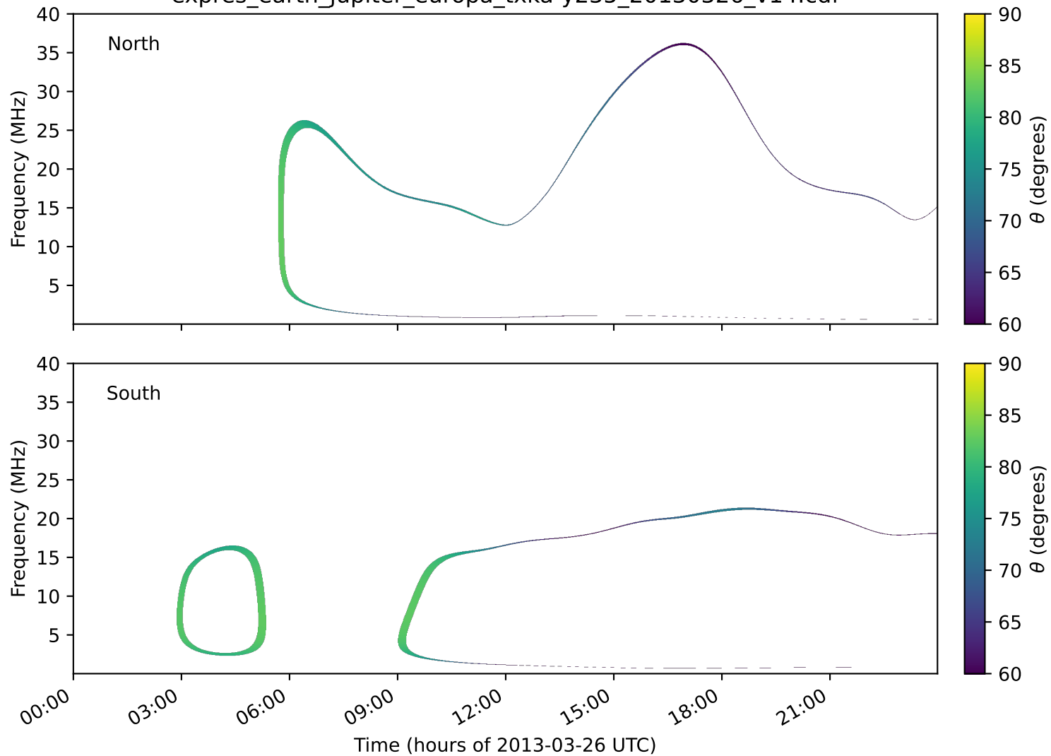
expres_earth_jupiter_europa_txka-y235_20130326_v14.cdf
