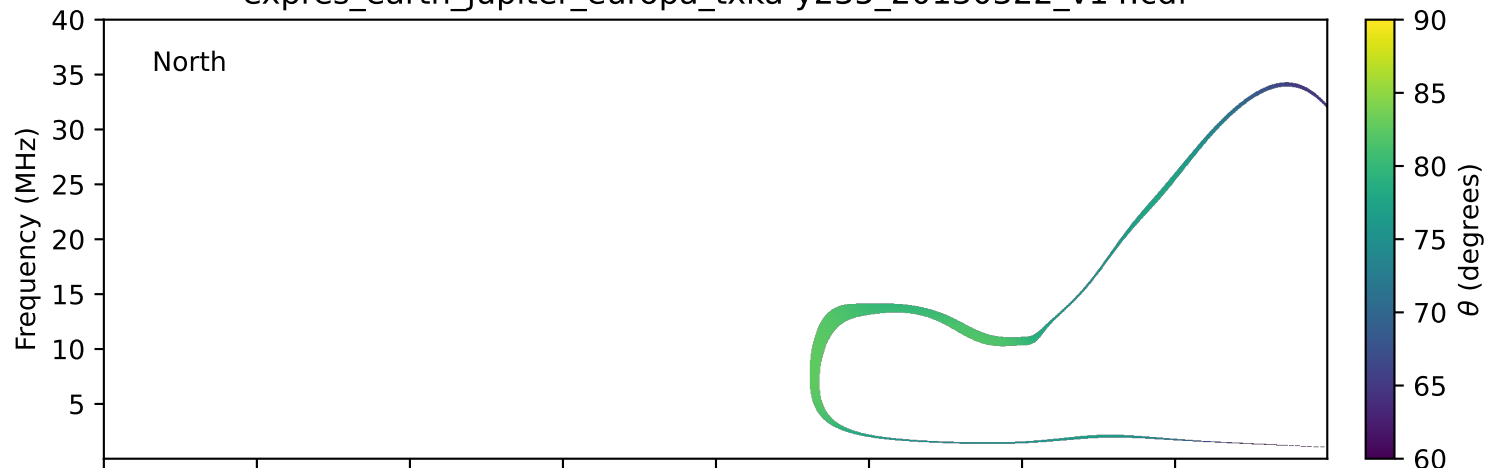
expres_earth_jupiter_europa_txka-y235_20130322_v14.cdf
