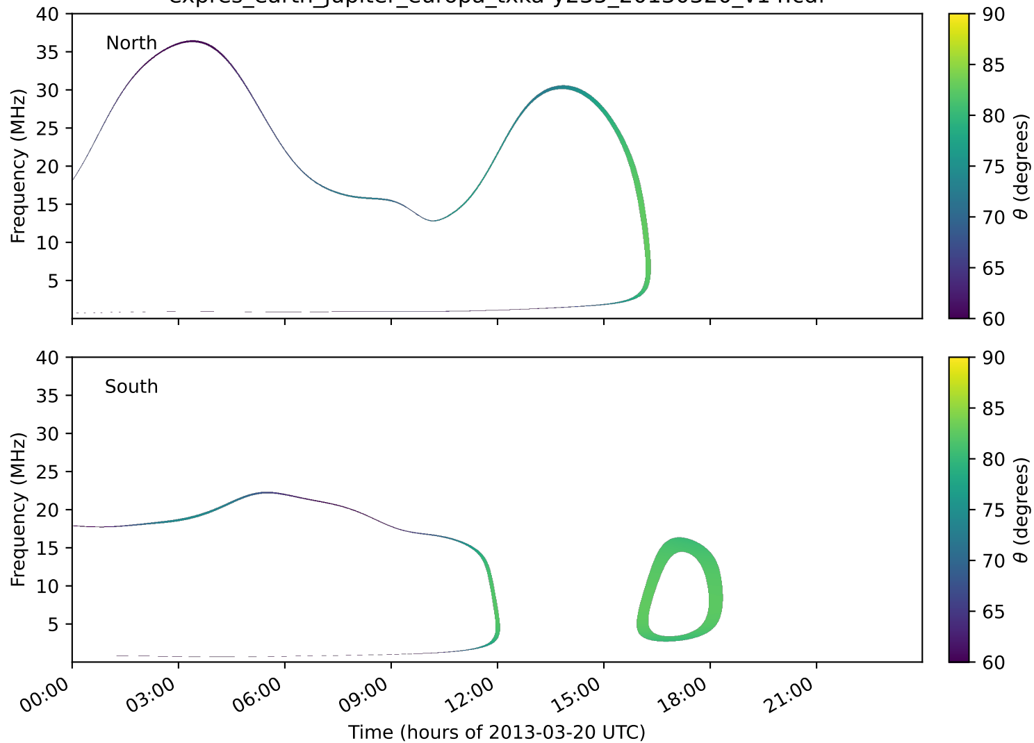
expres_earth_jupiter_europa_txka-y235_20130320_v14.cdf
