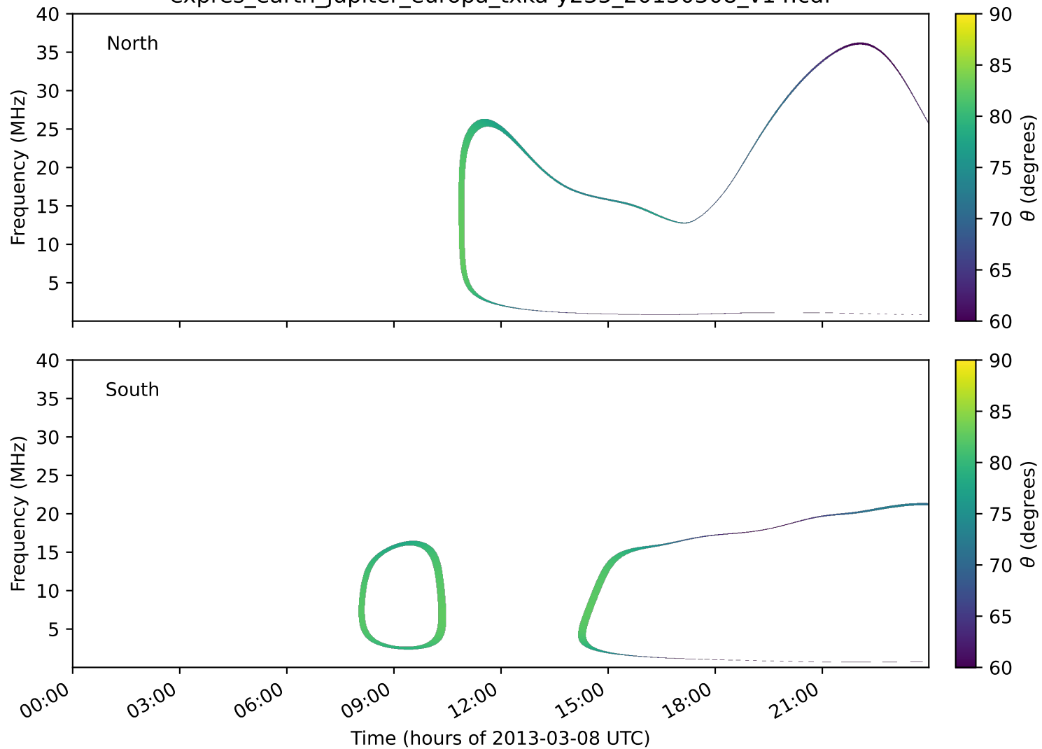
expres_earth_jupiter_europa_txka-y235_20130308_v14.cdf
