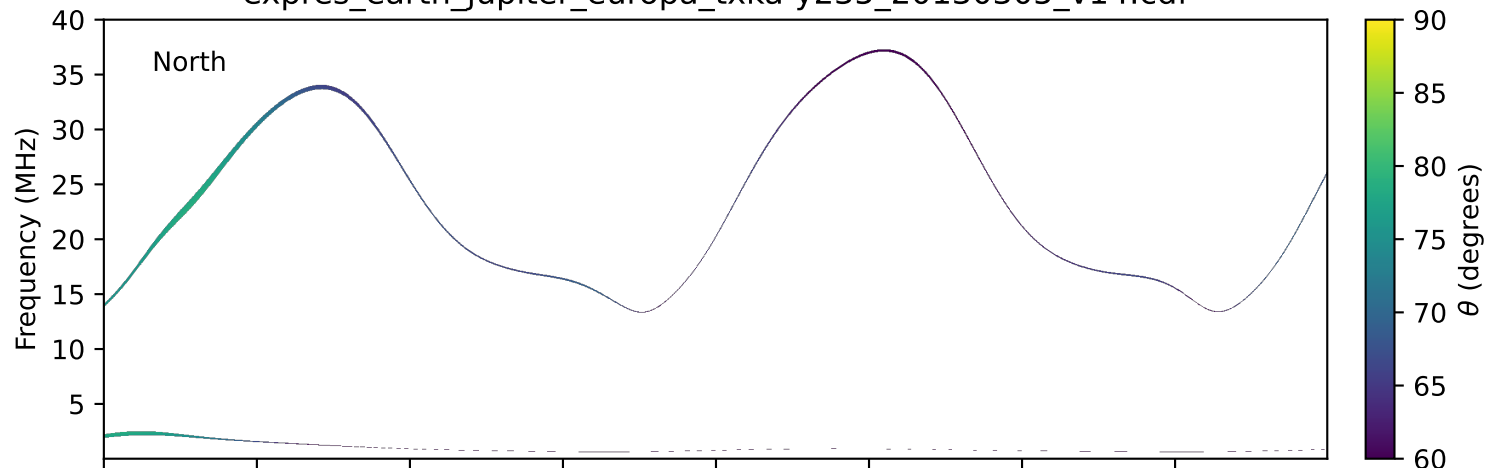
expres_earth_jupiter_europa_txka-y235_20130305_v14.cdf
