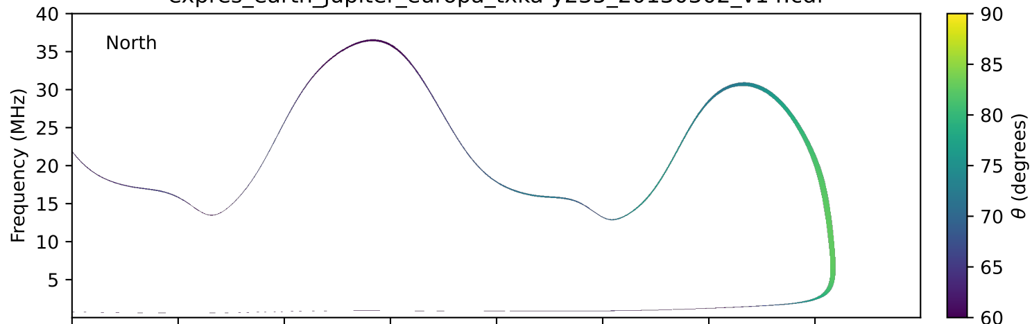
expres_earth_jupiter_europa_txka-y235_20130302_v14.cdf
