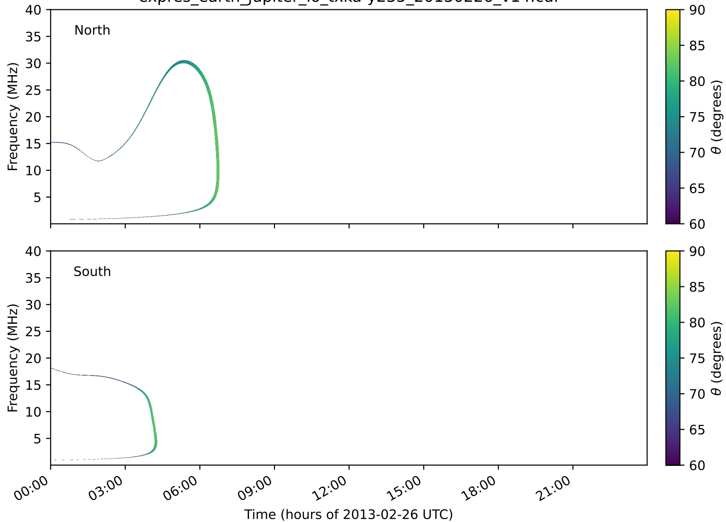
expres_earth_jupiter_io_txka-y235_20130226_v14.cdf
