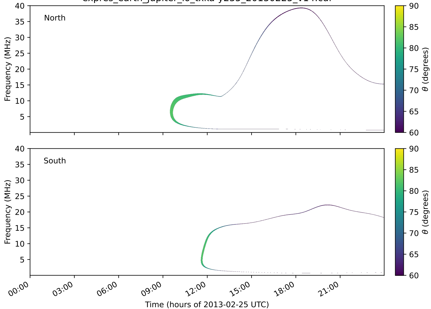
expres_earth_jupiter_io_txka-y235_20130225_v14.cdf
