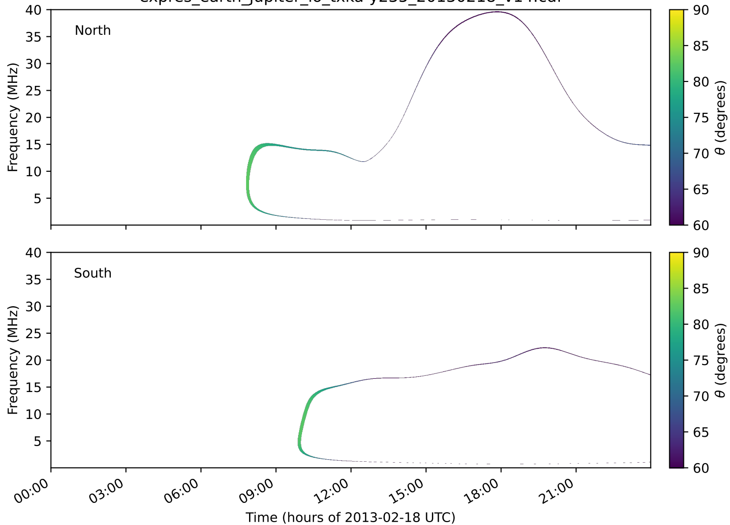
expres_earth_jupiter_io_txka-y235_20130218_v14.cdf
