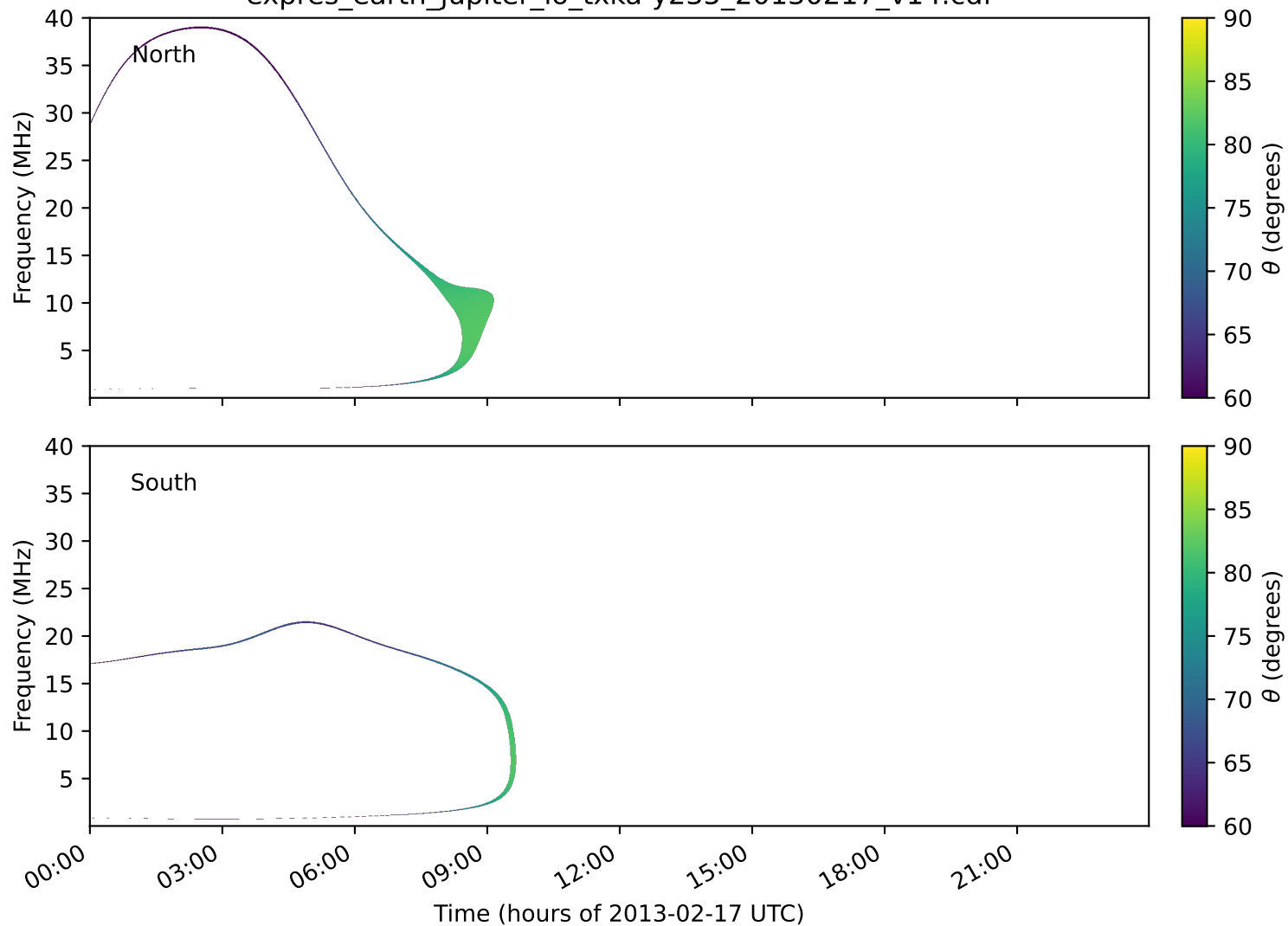
expres_earth_jupiter_io_txka-y235_20130217_v14.cdf
