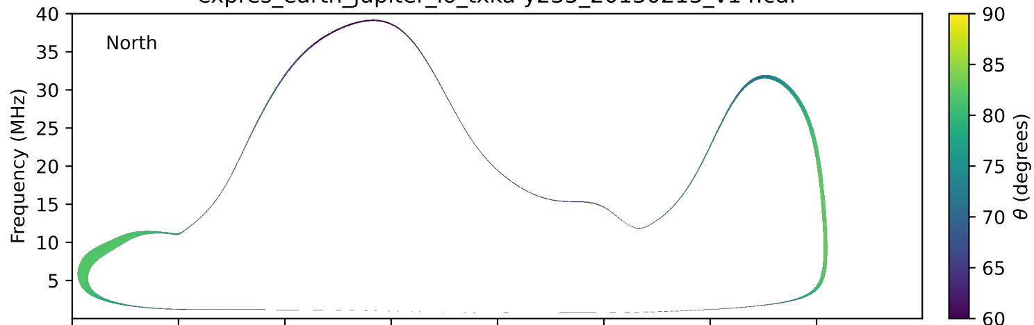
expres_earth_jupiter_io_txka-y235_20130213_v14.cdf
