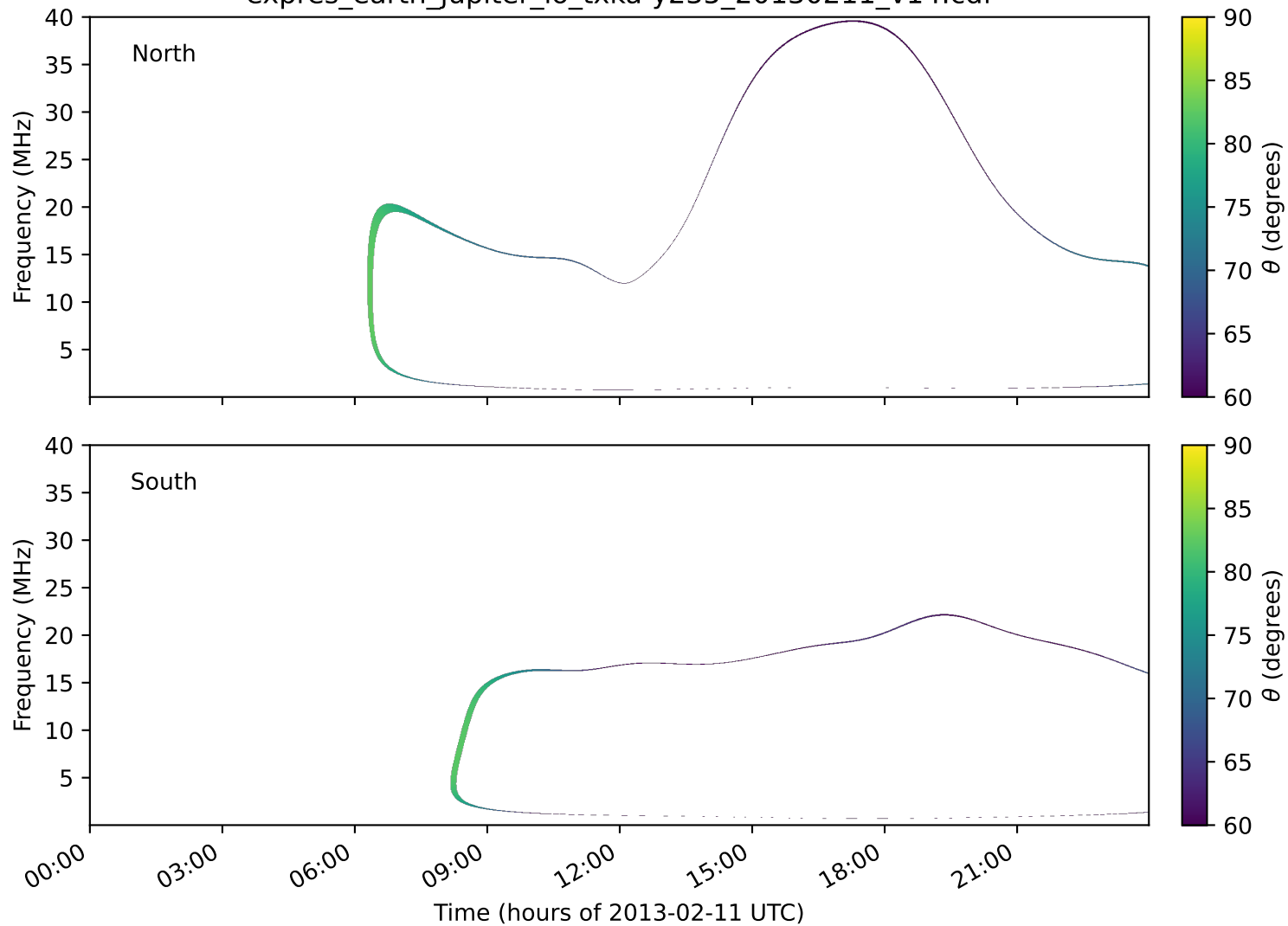
expres_earth_jupiter_io_txka-y235_20130211_v14.cdf
