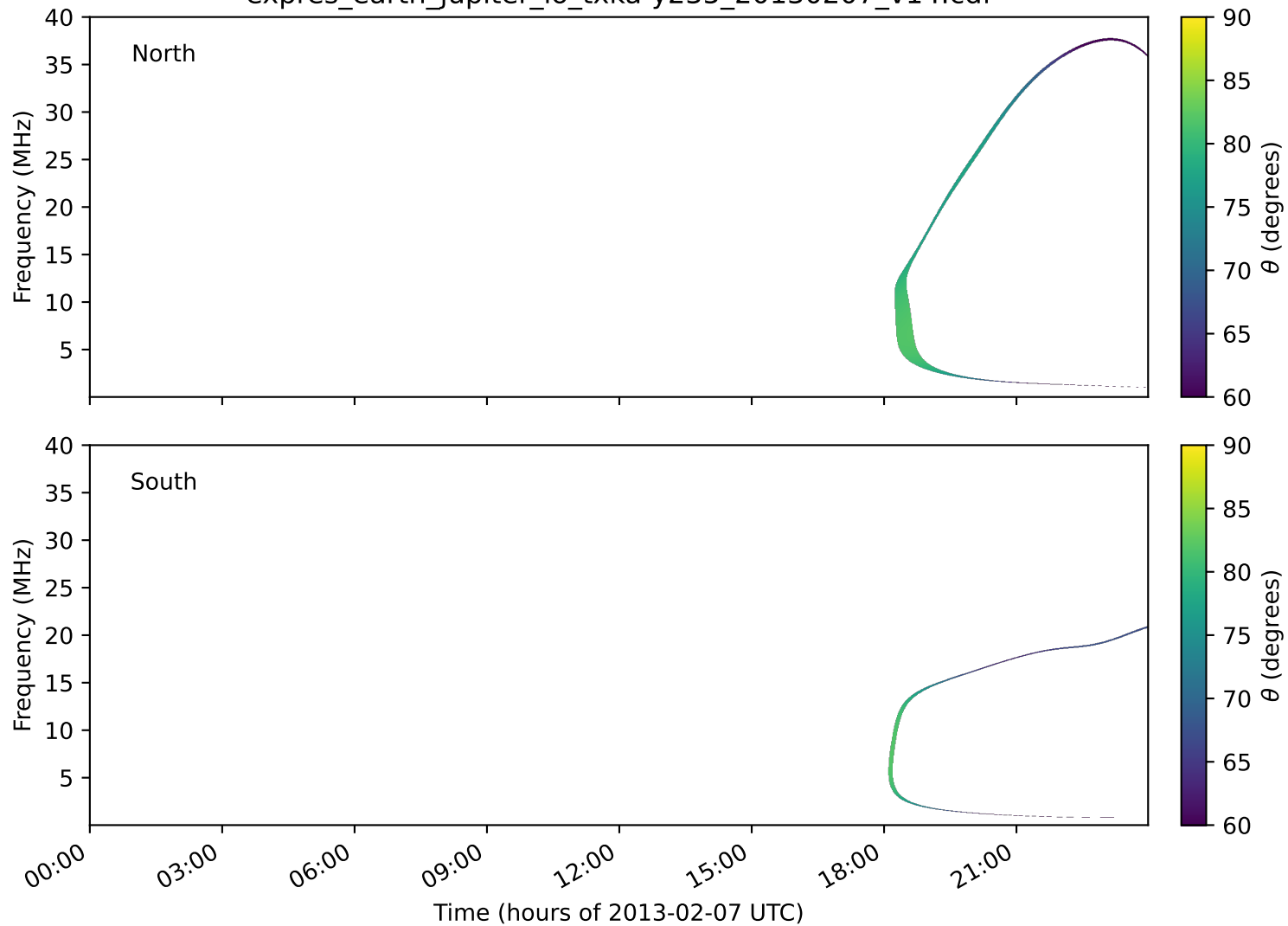
expres_earth_jupiter_io_txka-y235_20130207_v14.cdf
