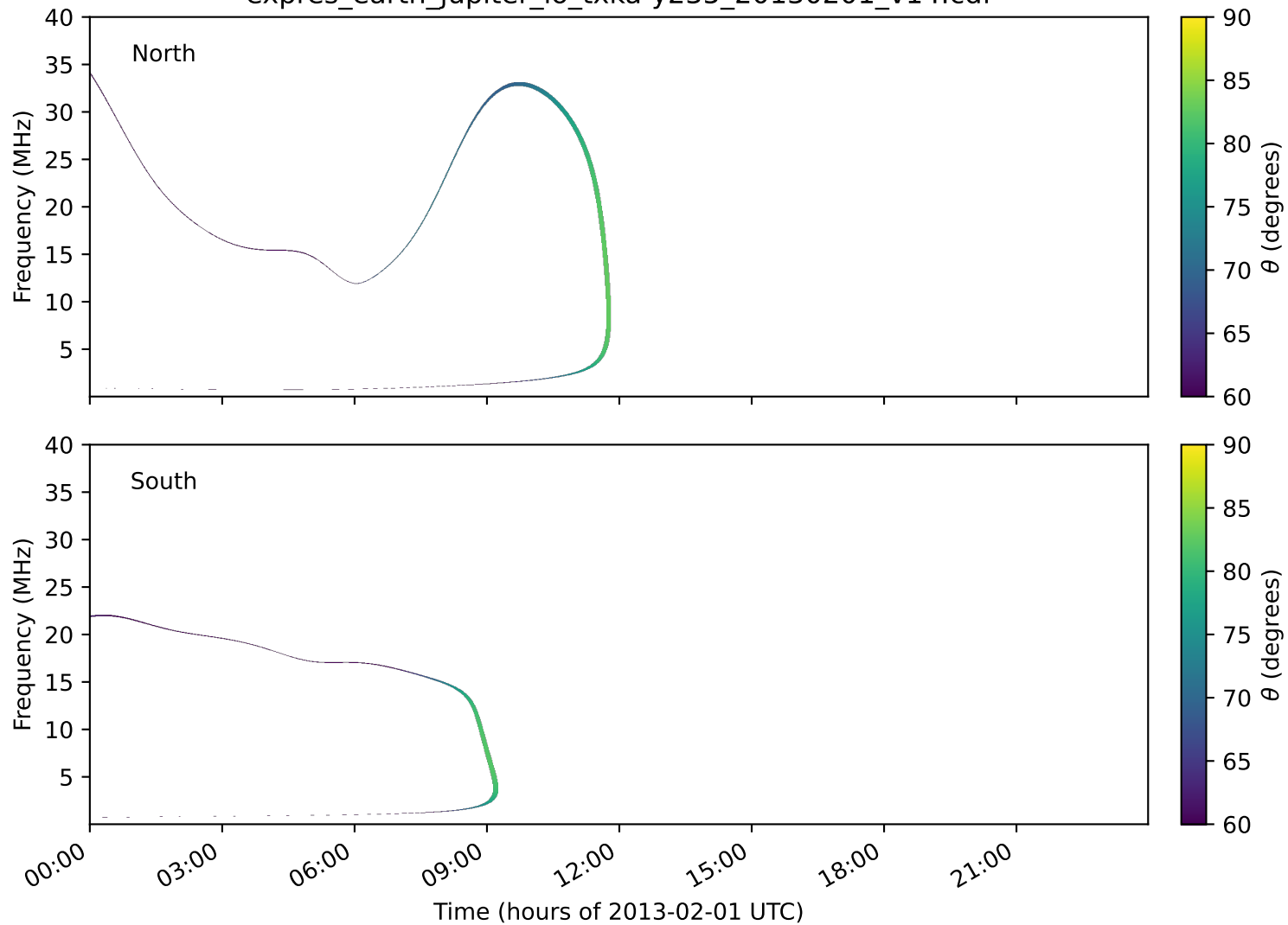
expres_earth_jupiter_io_txka-y235_20130201_v14.cdf
