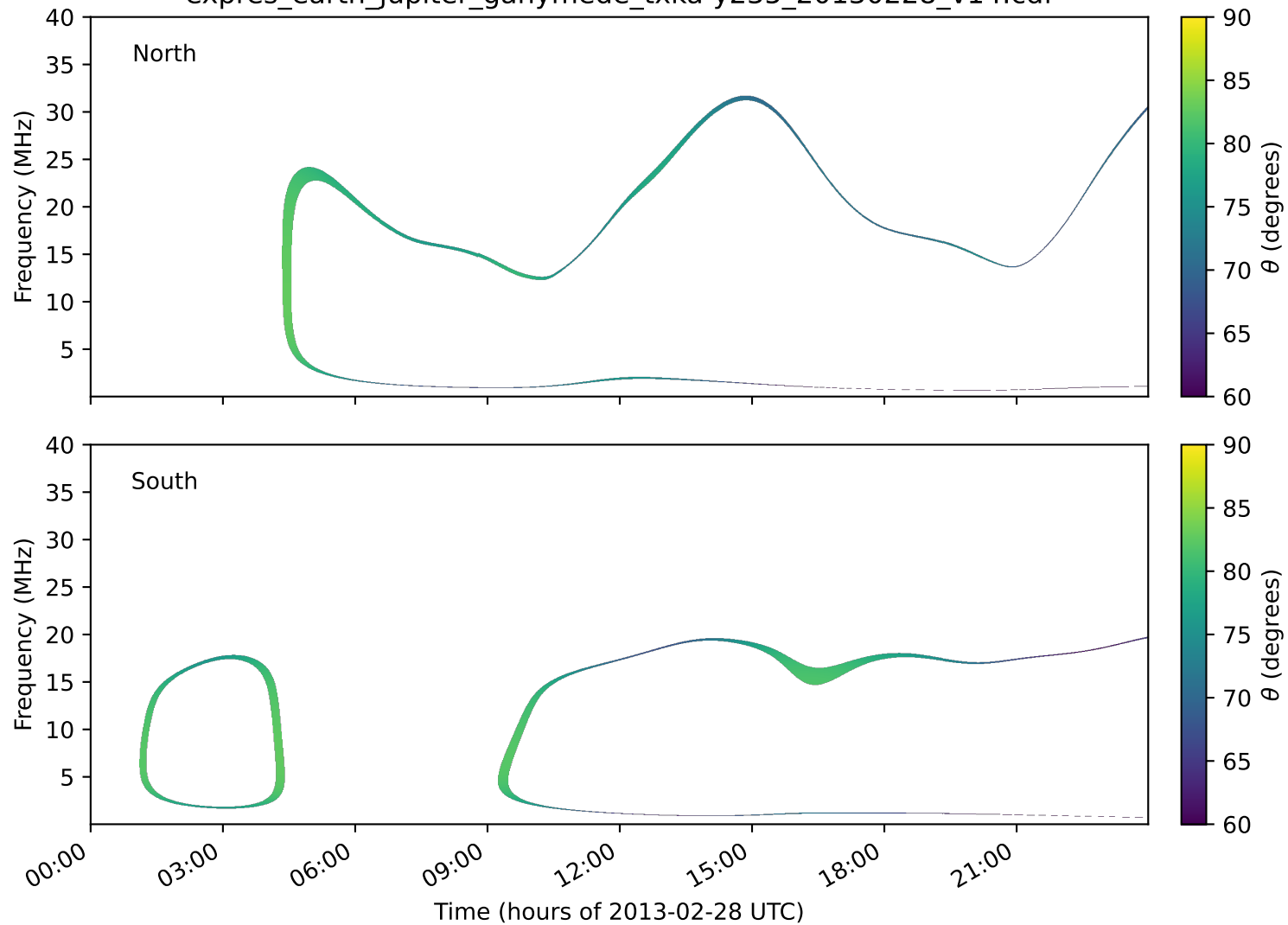
expres_earth_jupiter_ganymede_txka-y235_20130228_v14.cdf
