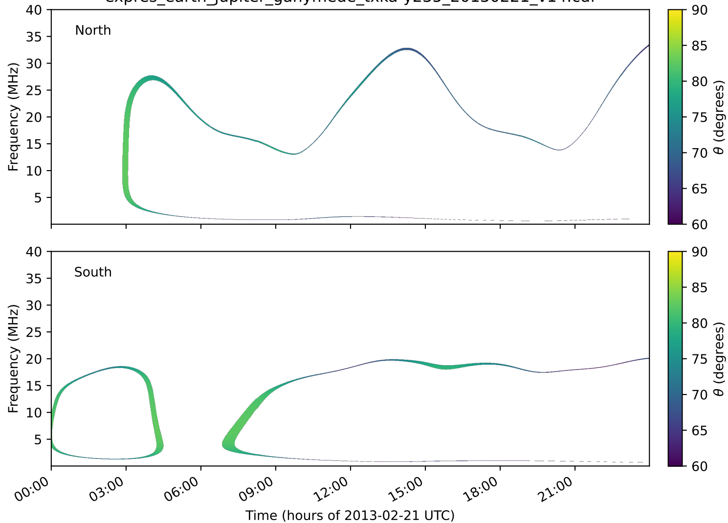
expres_earth_jupiter_ganymede_txka-y235_20130221_v14.cdf
