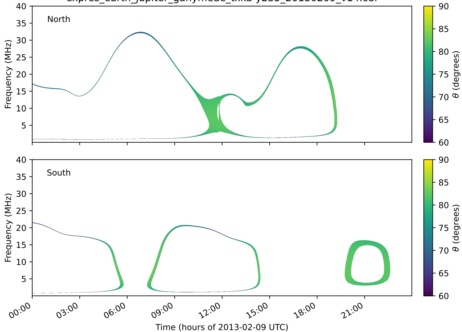
expres_earth_jupiter_ganymede_txka-y235_20130209_v14.cdf
