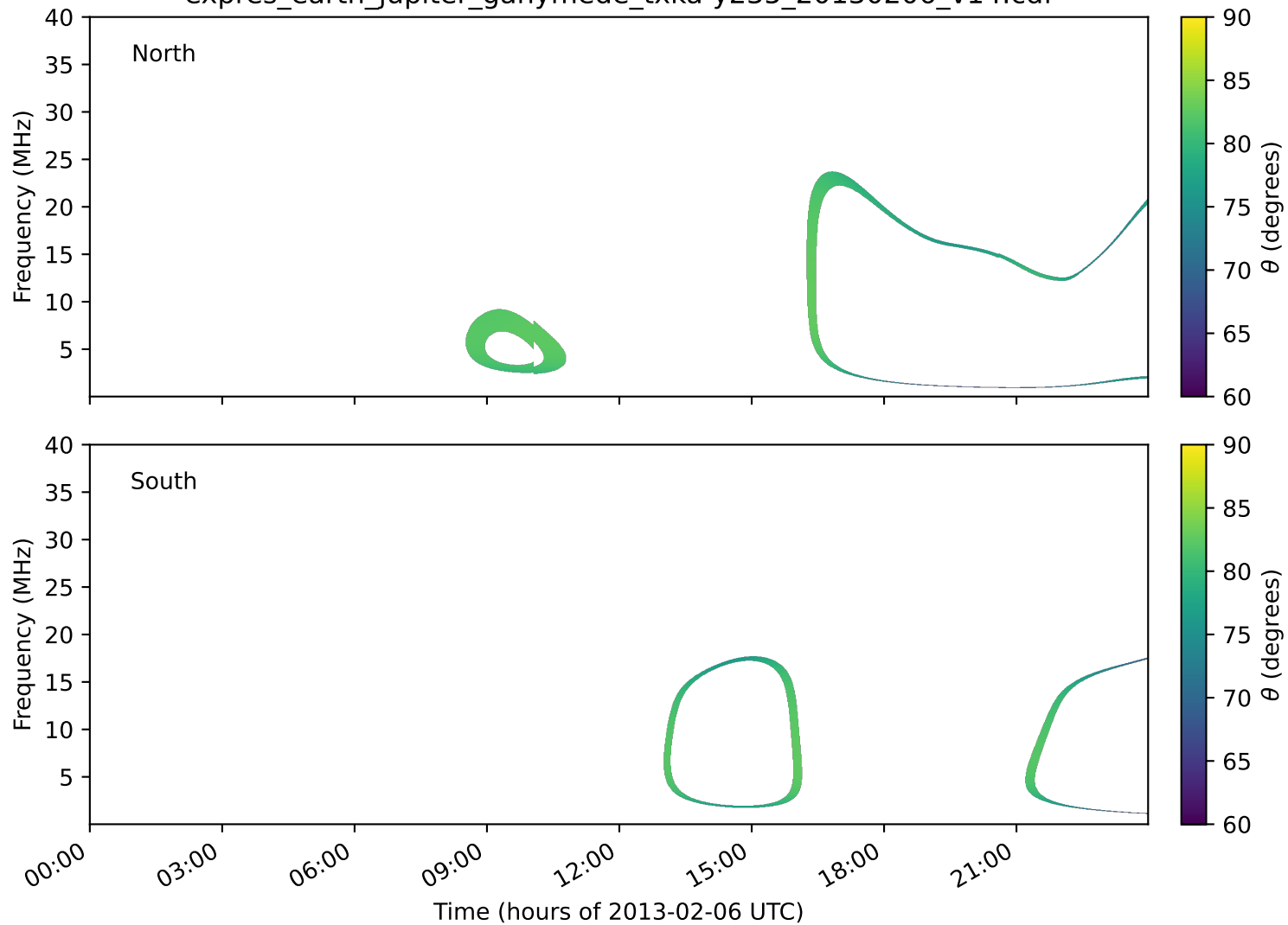
expres_earth_jupiter_ganymede_txka-y235_20130206_v14.cdf
