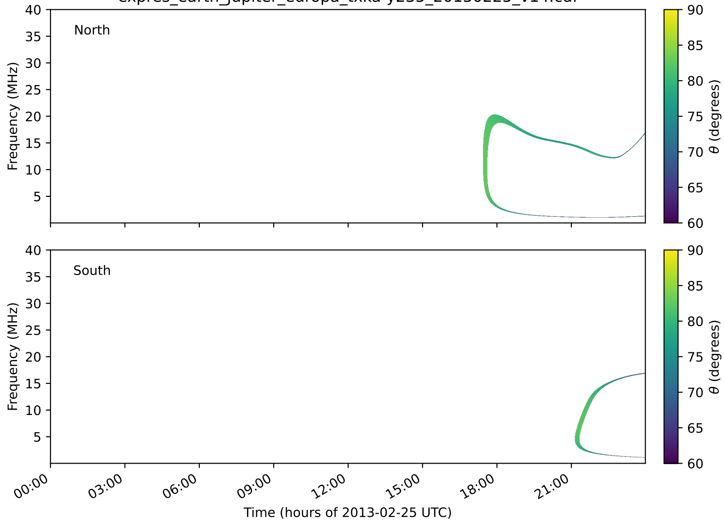
expres_earth_jupiter_europa_txka-y235_20130225_v14.cdf
