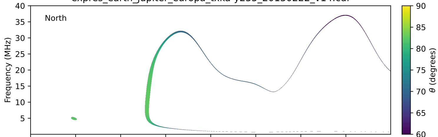
expres_earth_jupiter_europa_txka-y235_20130222_v14.cdf
