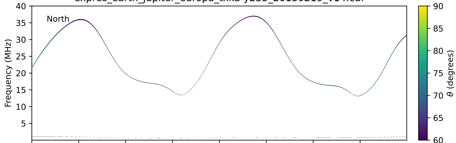
expres_earth_jupiter_europa_txka-y235_20130219_v14.cdf
