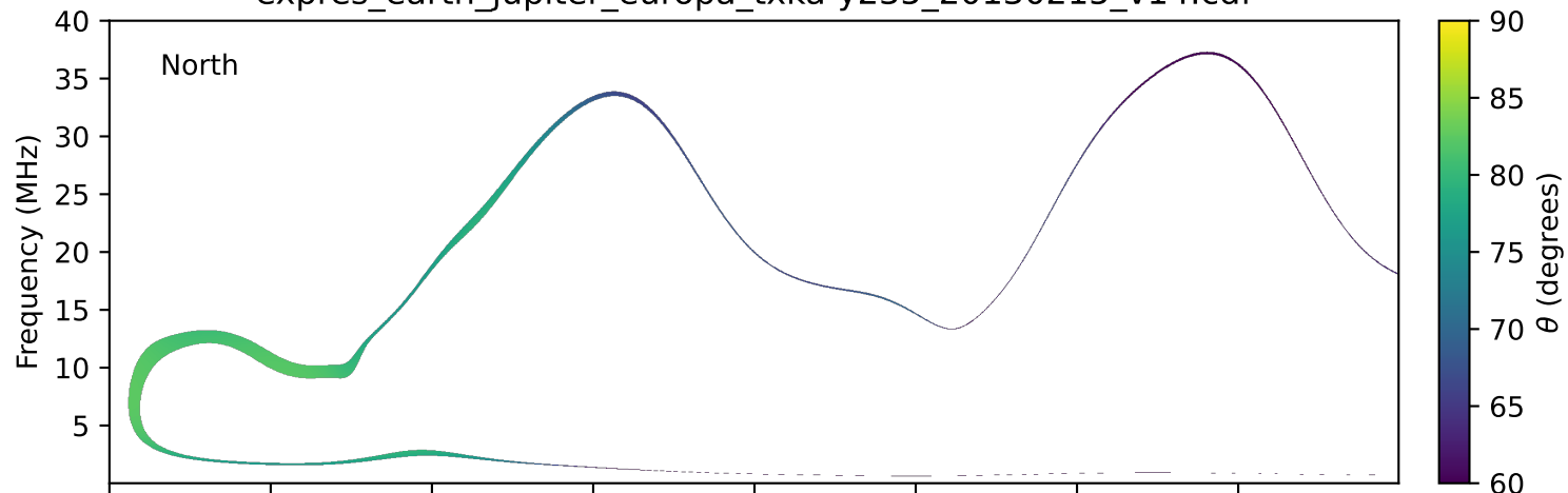
expres_earth_jupiter_europa_txka-y235_20130215_v14.cdf
