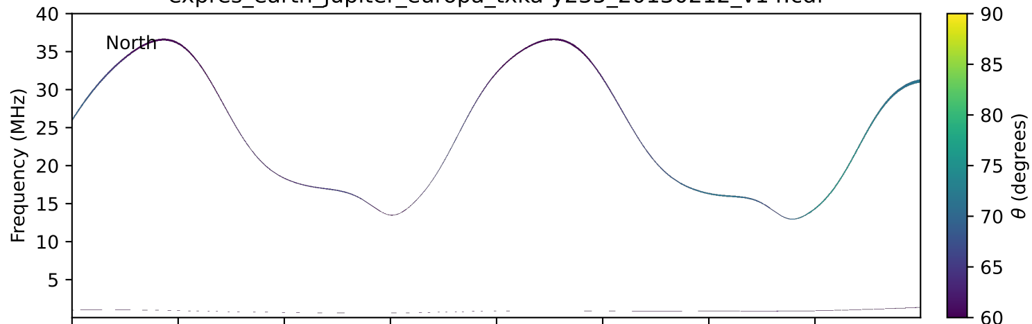
expres_earth_jupiter_europa_txka-y235_20130212_v14.cdf
