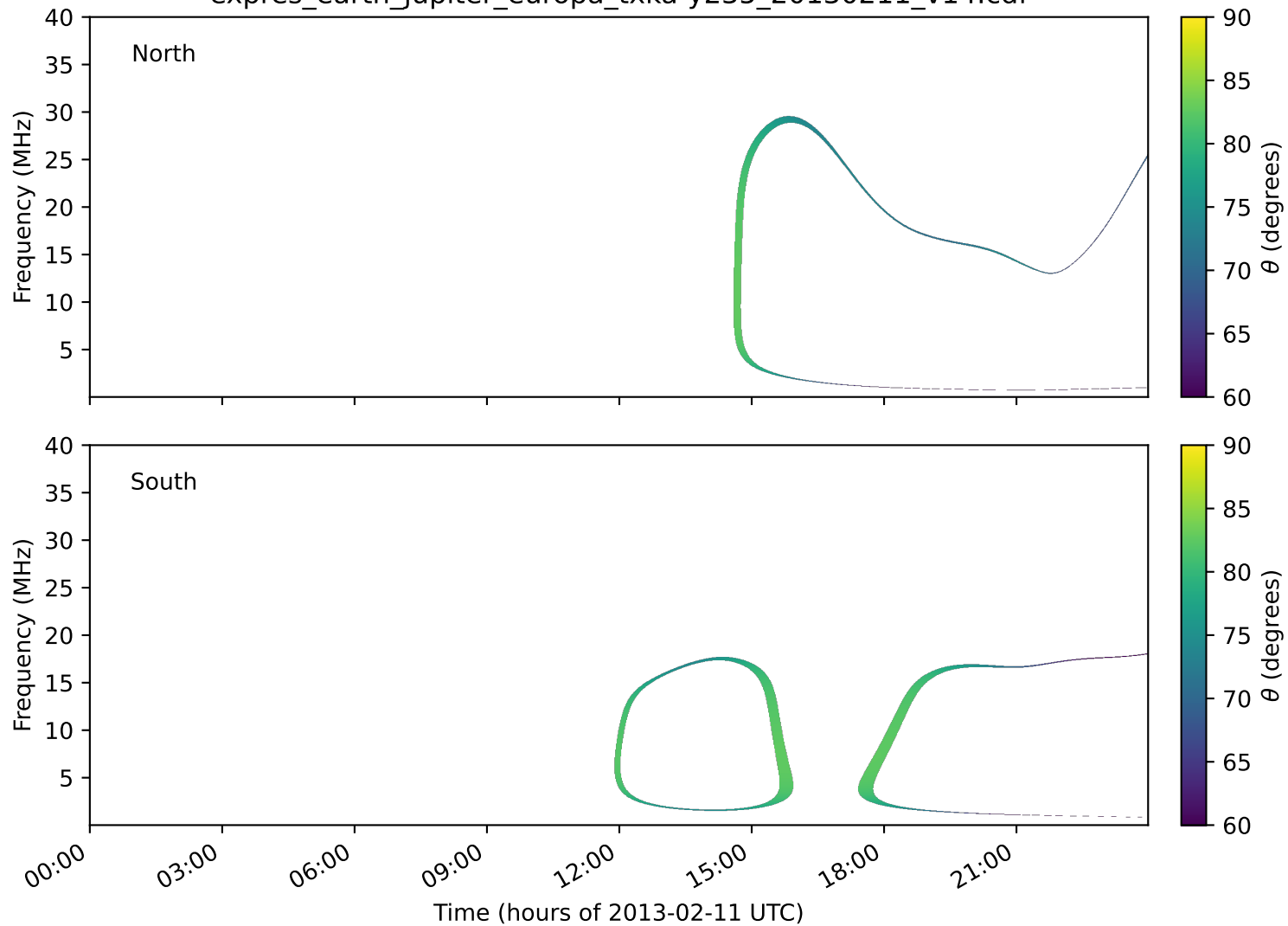
expres_earth_jupiter_europa_txka-y235_20130211_v14.cdf
