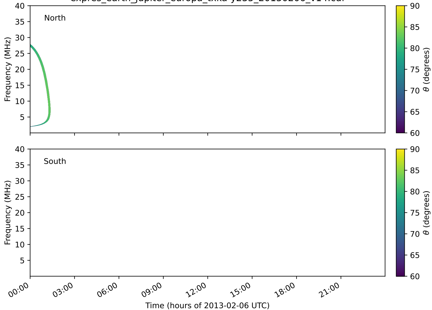
expres_earth_jupiter_europa_txka-y235_20130206_v14.cdf
