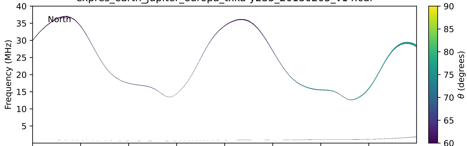
expres_earth_jupiter_europa_txka-y235_20130205_v14.cdf
