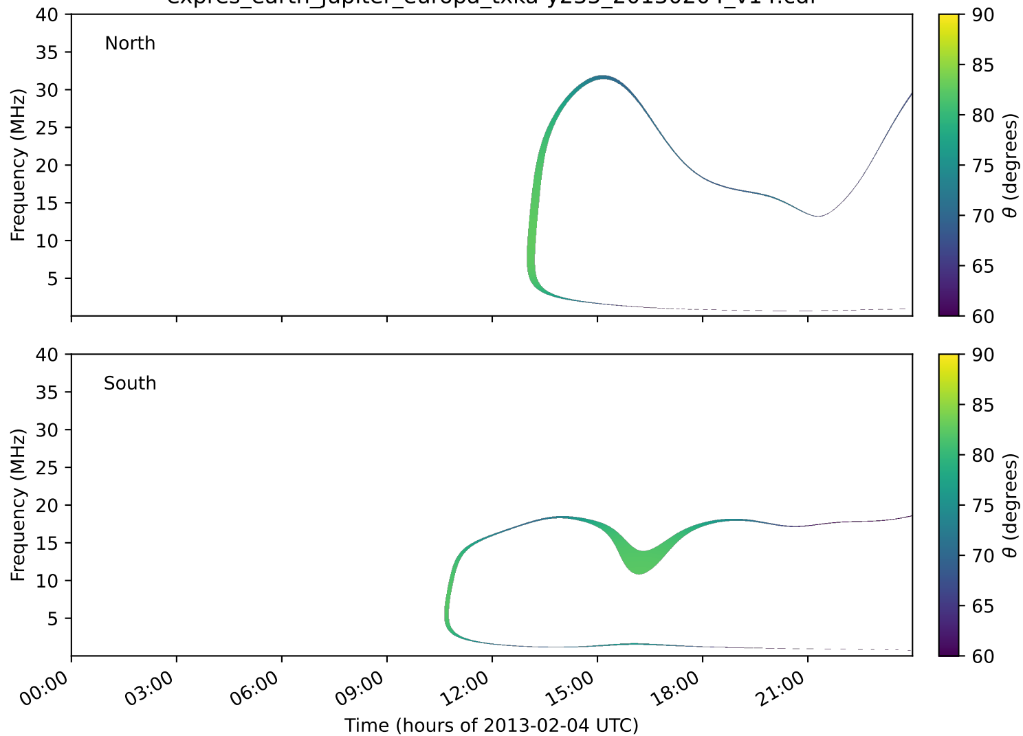
expres_earth_jupiter_europa_txka-y235_20130204_v14.cdf
