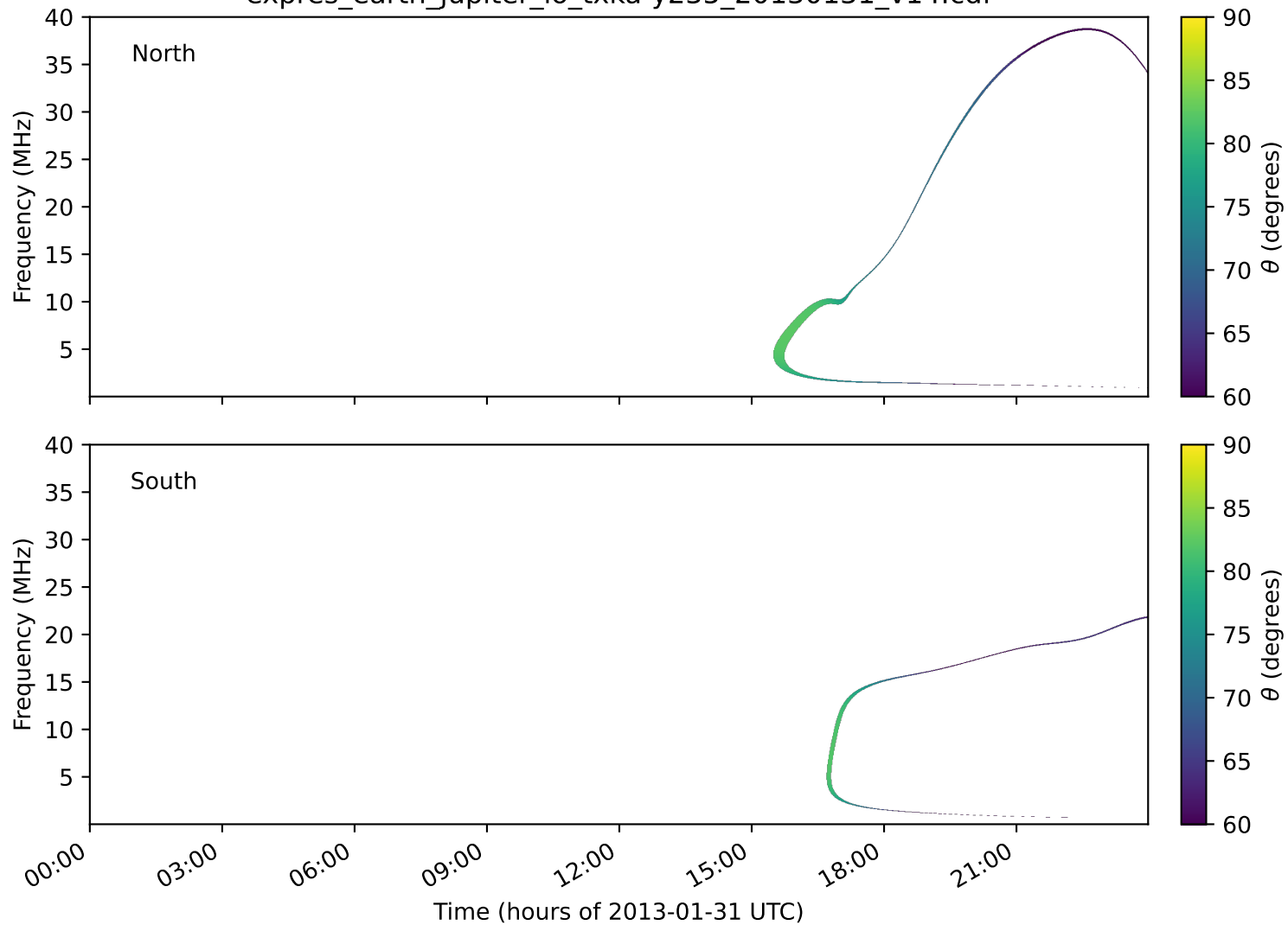
expres_earth_jupiter_io_txka-y235_20130131_v14.cdf
