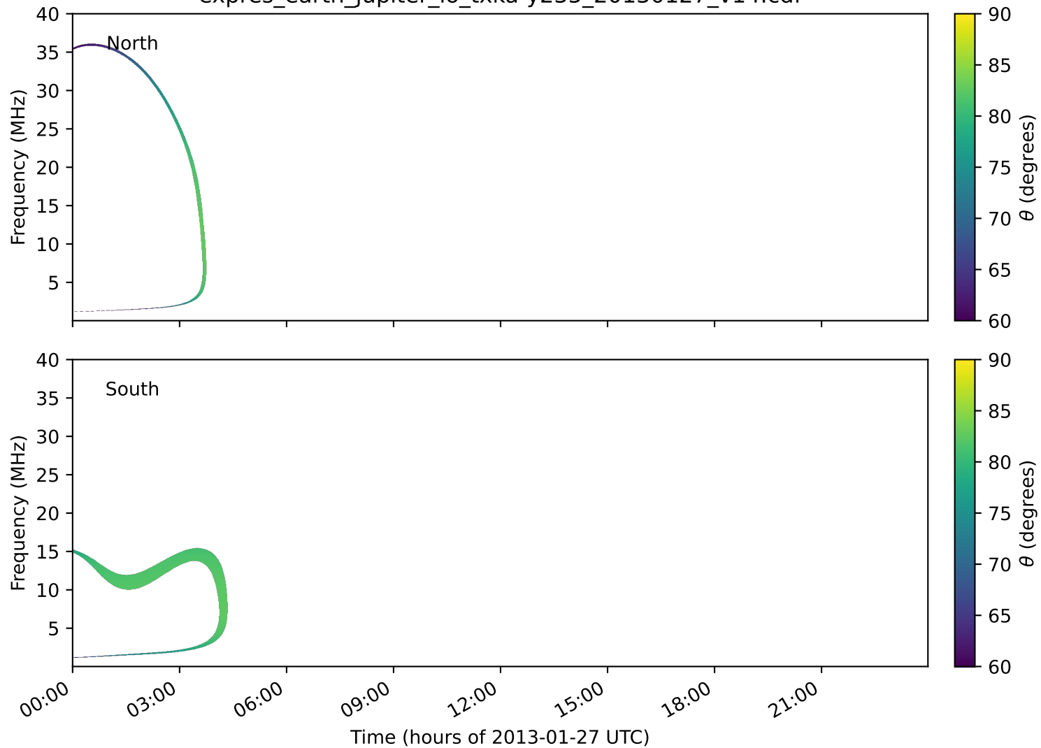
expres_earth_jupiter_io_txka-y235_20130127_v14.cdf
