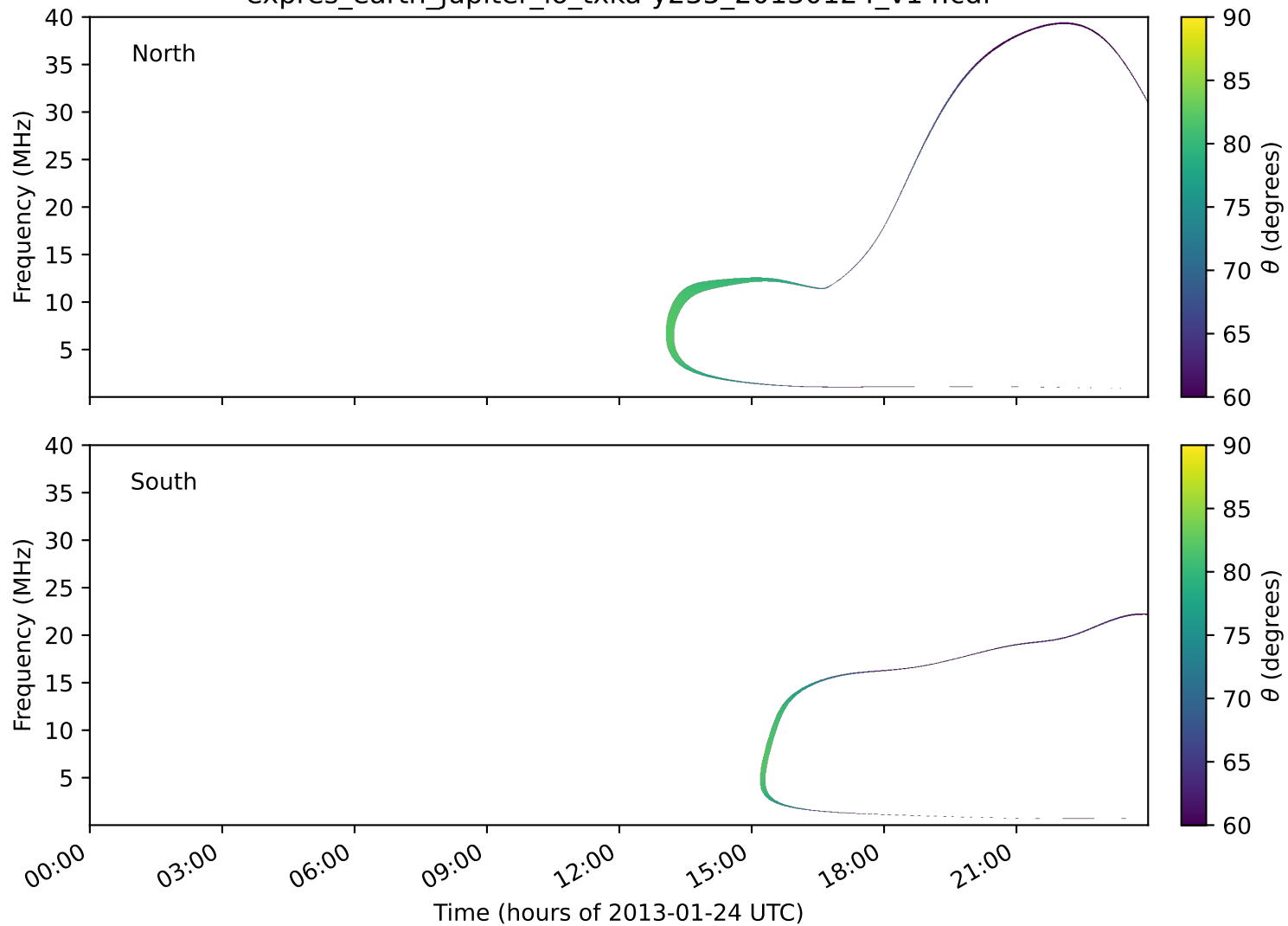
expres_earth_jupiter_io_txka-y235_20130124_v14.cdf
