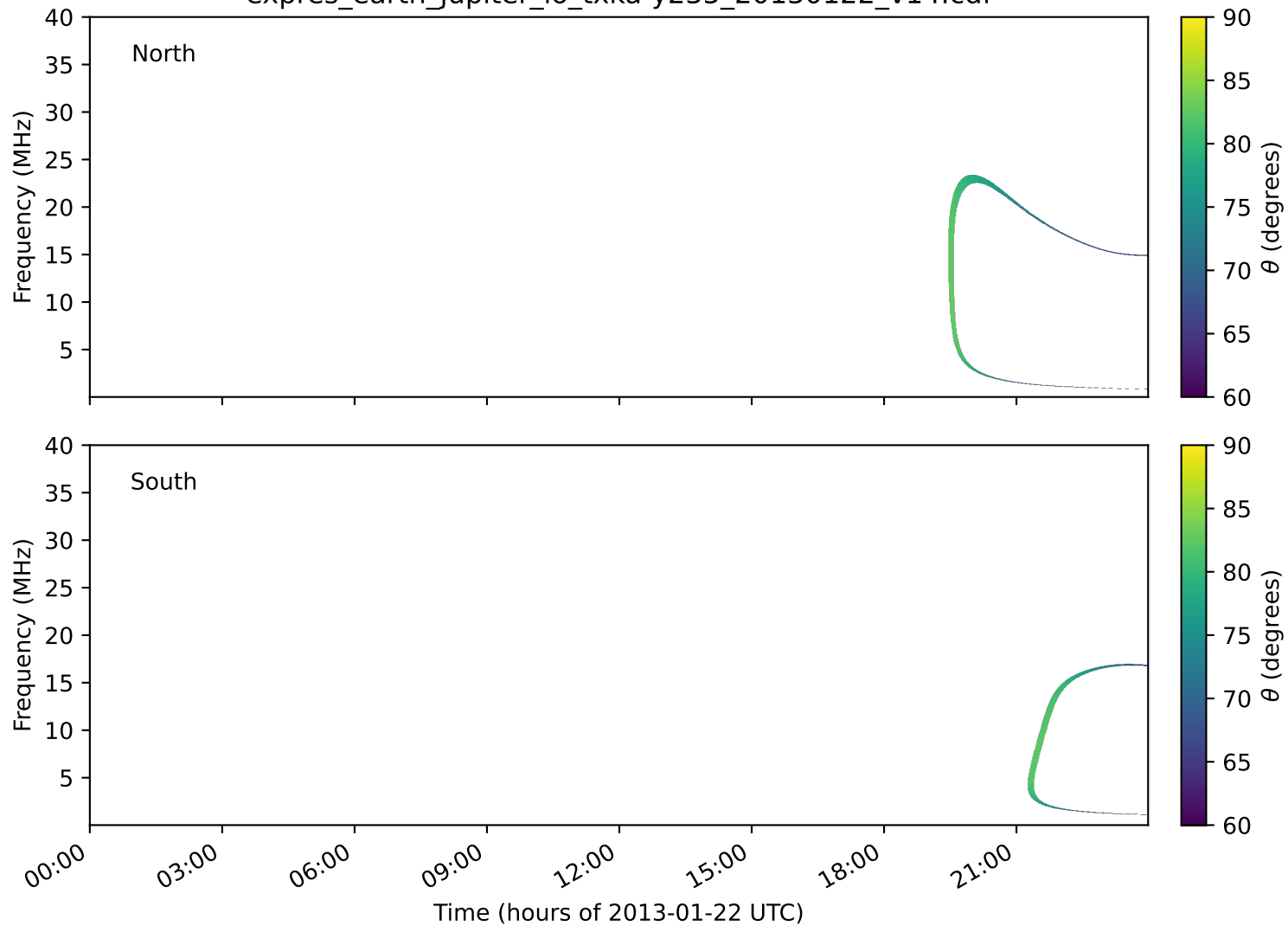
expres_earth_jupiter_io_txka-y235_20130122_v14.cdf
