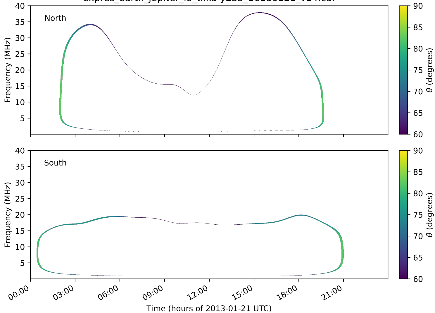
expres_earth_jupiter_io_txka-y235_20130121_v14.cdf
