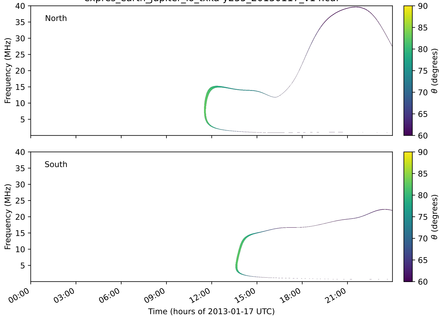
expres_earth_jupiter_io_txka-y235_20130117_v14.cdf
