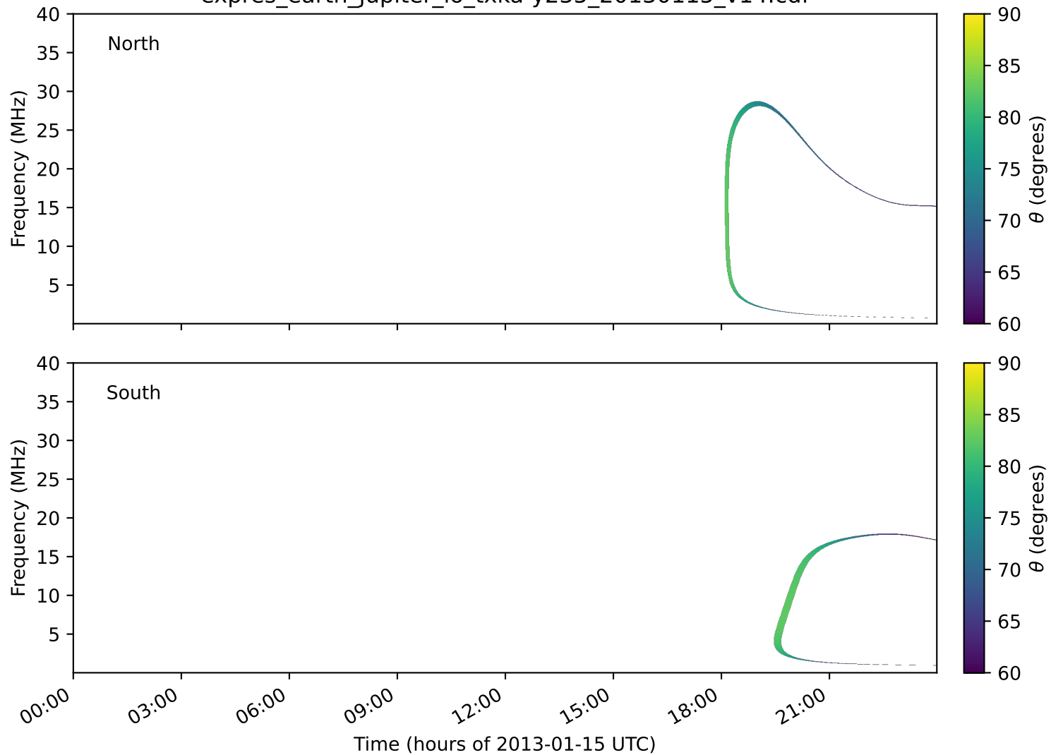
expres_earth_jupiter_io_txka-y235_20130115_v14.cdf
