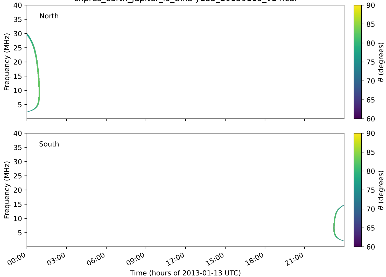
expres_earth_jupiter_io_txka-y235_20130113_v14.cdf
