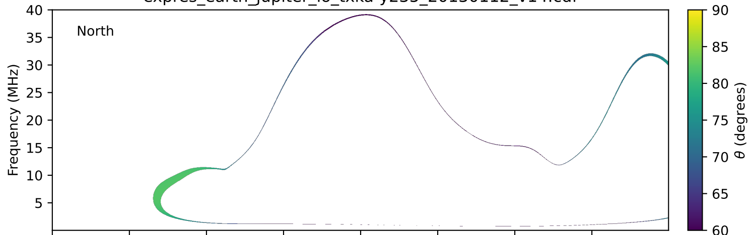
expres_earth_jupiter_io_txka-y235_20130112_v14.cdf
