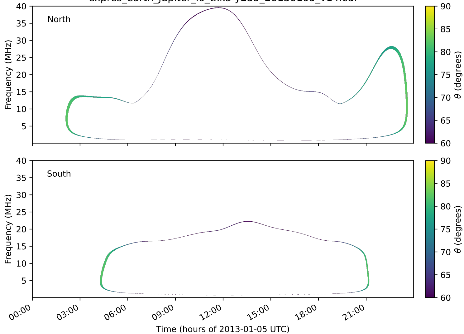
expres_earth_jupiter_io_txka-y235_20130105_v14.cdf
