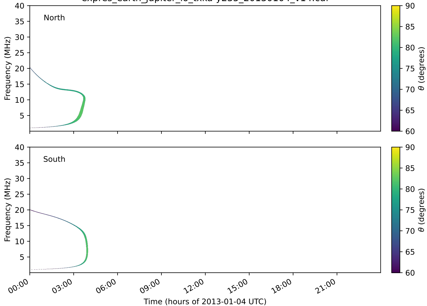
expres_earth_jupiter_io_txka-y235_20130104_v14.cdf
