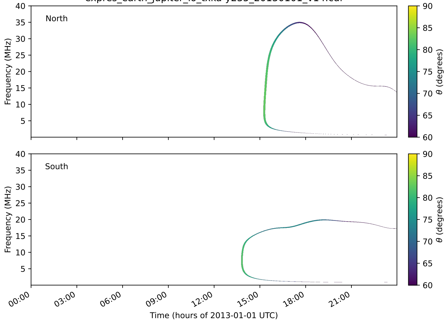
expres_earth_jupiter_io_txka-y235_20130101_v14.cdf
