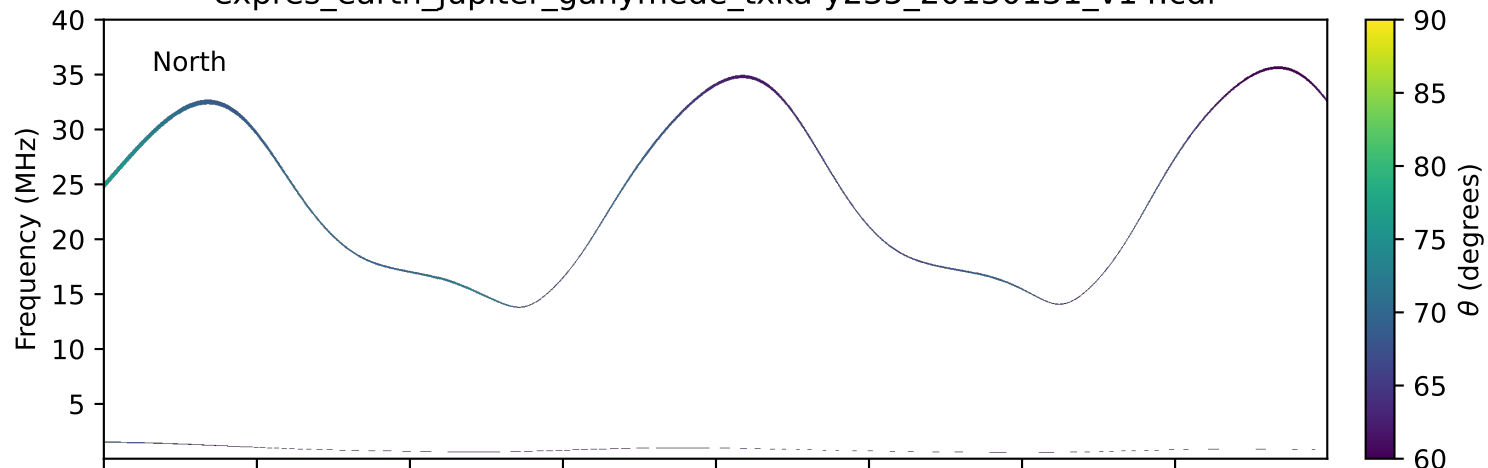
expres_earth_jupiter_ganymede_txka-y235_20130131_v14.cdf
