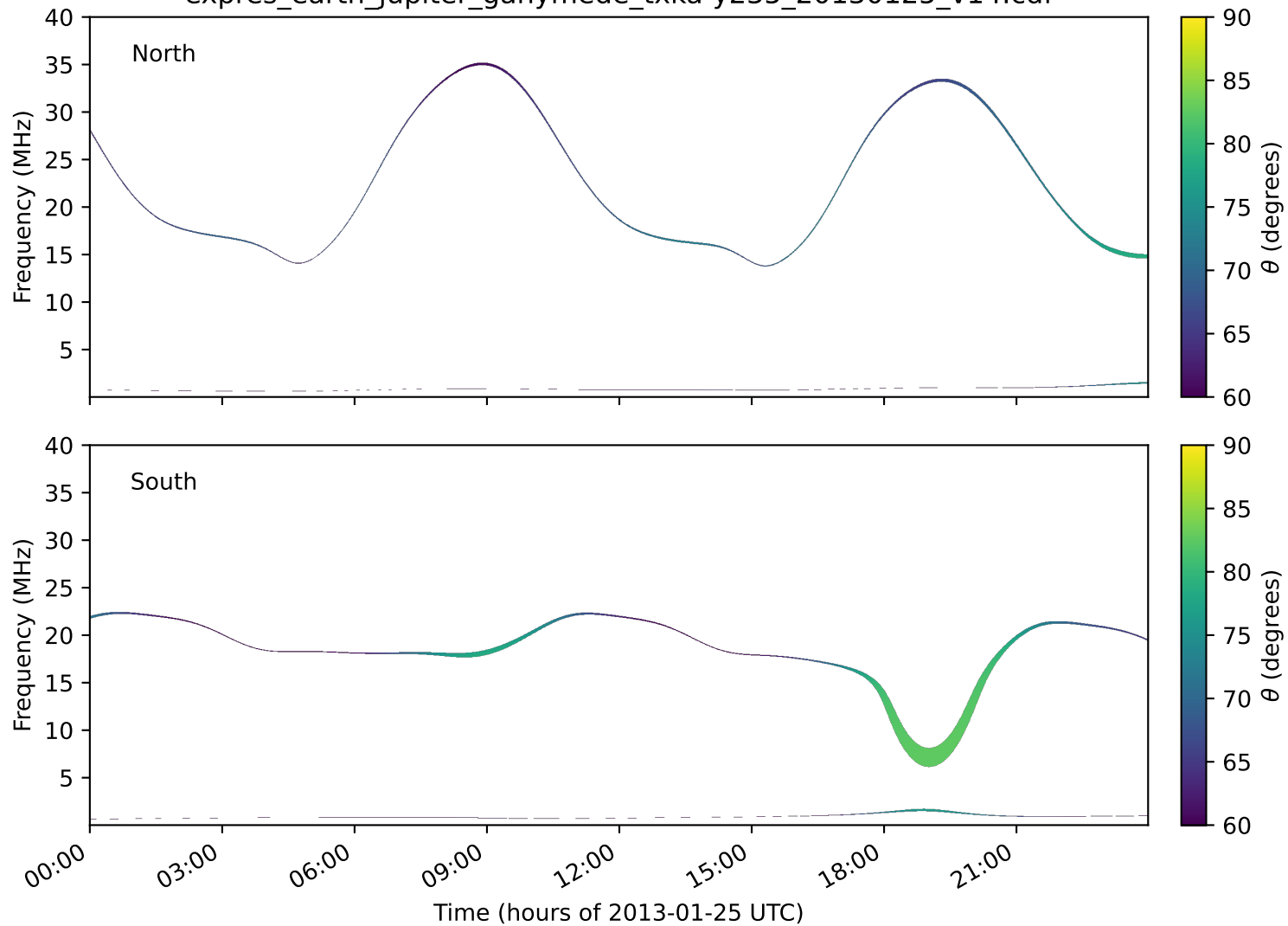
expres_earth_jupiter_ganymede_txka-y235_20130125_v14.cdf
