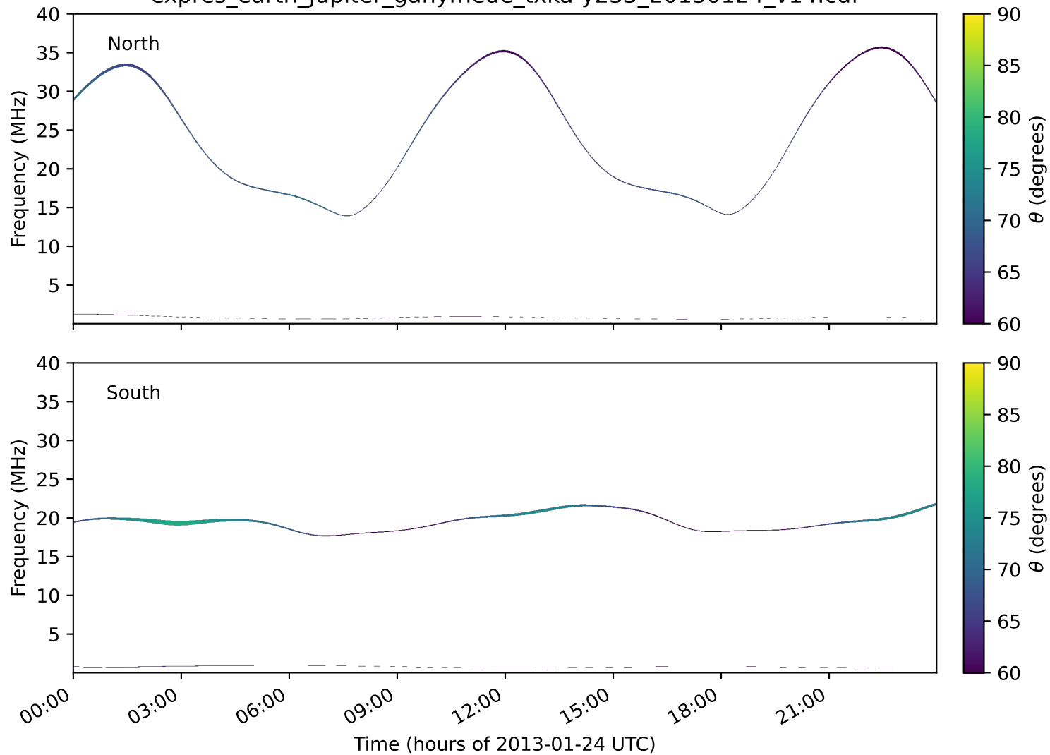
expres_earth_jupiter_ganymede_txka-y235_20130124_v14.cdf
