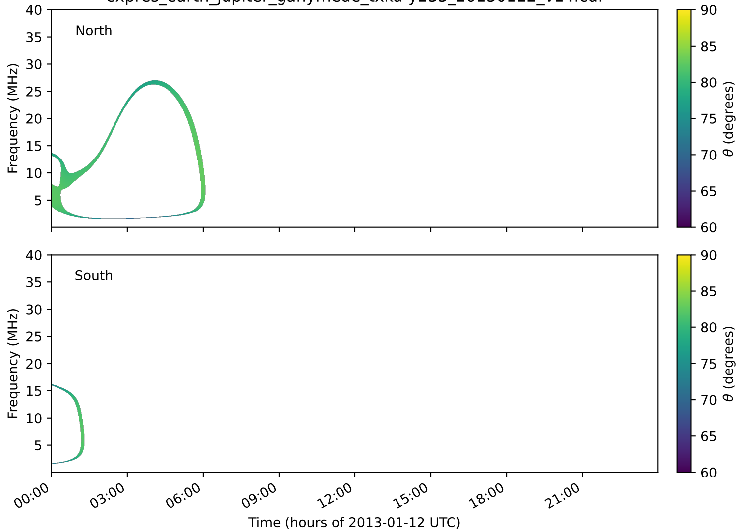
expres_earth_jupiter_ganymede_txka-y235_20130112_v14.cdf
