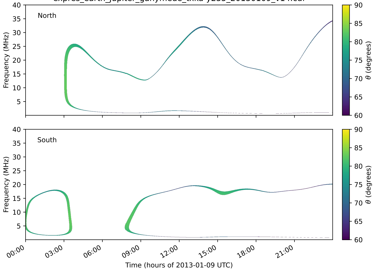
expres_earth_jupiter_ganymede_txka-y235_20130109_v14.cdf
