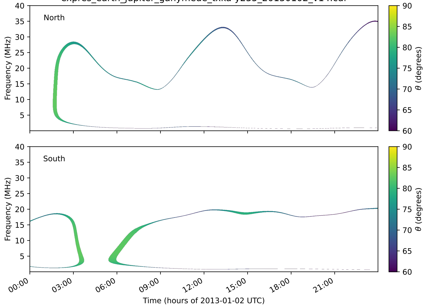
expres_earth_jupiter_ganymede_txka-y235_20130102_v14.cdf
