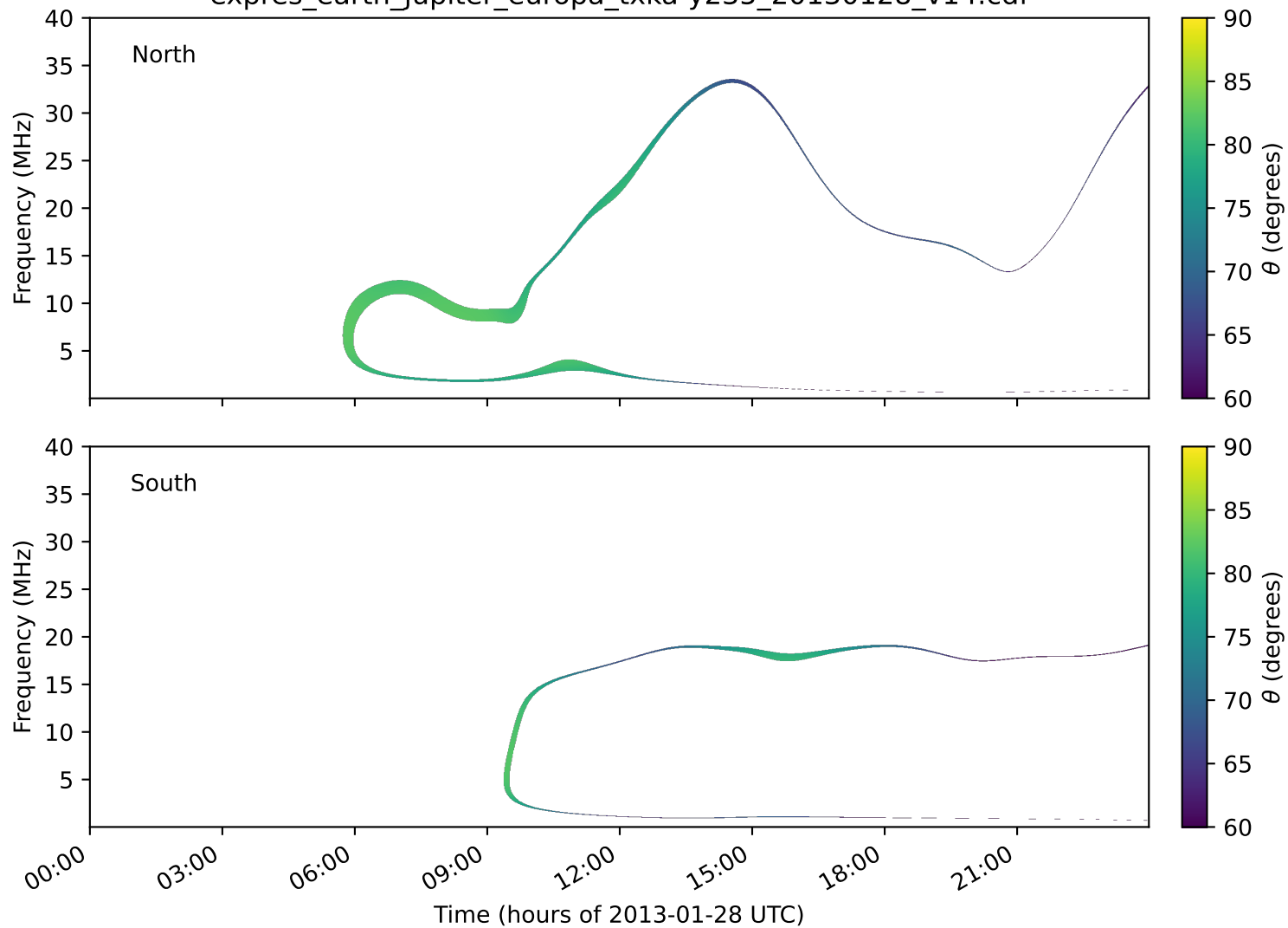
expres_earth_jupiter_europa_txka-y235_20130128_v14.cdf
